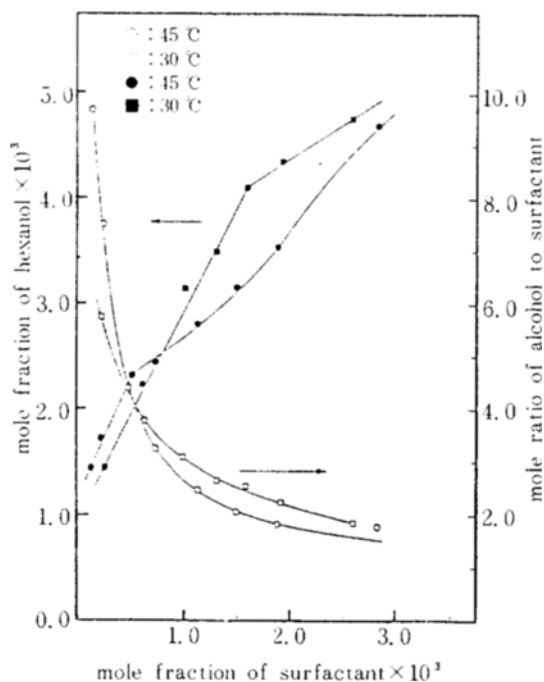
Fig. 7. Solubility limits and alcohol/surfactant ratio of sodium dodecyl sulfate-1-hexanol-water systems in the water-continuous phase at 30°C and 45°C.
